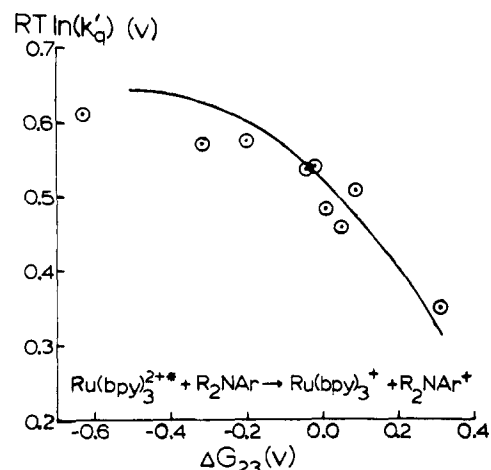
Figure 3. Plot of RT \ln k'_q vs. \Delta G_{23} in \text{CH}_3\text{CN} ( \mu = 0.1 \text{ M} ) at 22 \pm 2^\circ \text{C} for the quenching of \text{Ru}(\text{bpy})_3^{2+*} by \text{R}_2\text{NAr} . The theoretical line was drawn using eq 12, k'_q(0) = 8.8 \times 10^6 \text{ M}^{-1} \text{ s}^{-1} , and \lambda = 11 \text{ kcal/mol} (0.48 V).
