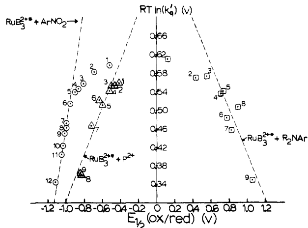
Figure 1. Plot of RT \ln k_q' (V) vs. E_{1/2}(\text{Ox/Red}) (V) in \text{CH}_3\text{CN} ( \mu = 0.1 M) at 22 \pm 2^\circ\text{C} for the quenching of \text{Ru}(\text{bpy})_3^{2+*} by \text{R}_2\text{NAr} ( \square ), \text{P}^{2+} ( \triangle ), and \text{ArNO}_2 ( \circ ). Data were taken from Tables I-III. Lines of slope = 1/2 are shown drawn through the experimental data for the \text{R}_2\text{NAr} and \text{P}^{2+} points and a line of slope = 1 through the \text{ArNO}_2 data.
