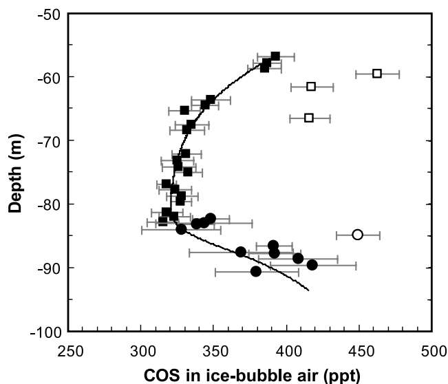
Figure 5. Carbonyl sulfide mixing ratios in air trapped in ice collected at Siple Dome, Antarctica, in December 1995 (81.65°S) (solid and open circles [Aydin et al. , 2002]) and additional measurements from this same core (solid and open squares (this work)). Points suspected of being contaminated were not included in model calculations (open symbols). Error bars represent measurement uncertainty (analysis uncertainty of \pm 1 standard deviation plus a blank uncertainty as described by Aydin et al. [2004]). The solid line is the depth profile calculated for COS in Siple Dome ice from the 350-year history, H3. The depth of the firn-to-ice transition at this site is 56 m.
