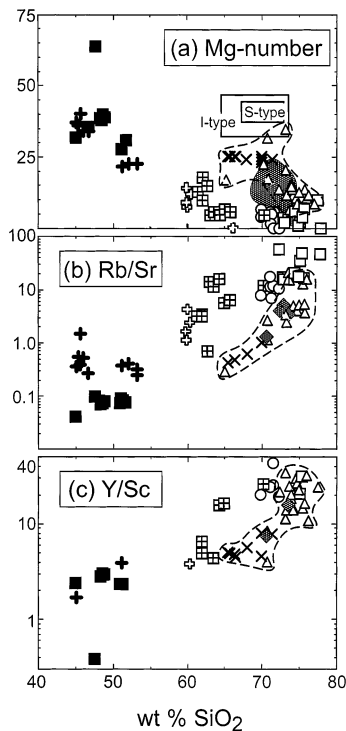
Fig. 4. (a) Mg-number ( 100 \times molar \text{Mg}/[\text{Mg} + \text{Fe}] ), (b) \log \text{Rb}/\text{Sr} and (c) \log \text{Y}/\text{Sc} versus wt% silica in Pikes Peak samples. Symbols as in Fig. 3. In (a), the shaded field represents the PPG (data from Barker et al., 1975). In (b) and (c), shaded diamonds represent the pink PPG (data from Table 9, this study). Ranges in Mg-number for I- and S-type granites are from Whalen et al. (1987). The dashed lines encircle samples of the potassic series analyzed here (Tables 8–10).
