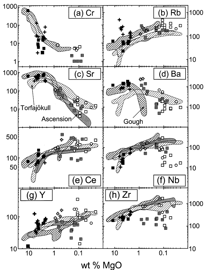
Fig. 14. Log-log plots of (a) Cr, (b) Rb, (c) Sr, (d) Ba, (e) Ce, (f) Nb, (g) Y and (h) Zr (ppm) versus MgO (wt%) in Pikes Peak sodic series rocks and selected ocean island suites. Symbols as in Fig. 3, and data sources and fields as in Fig. 13.
