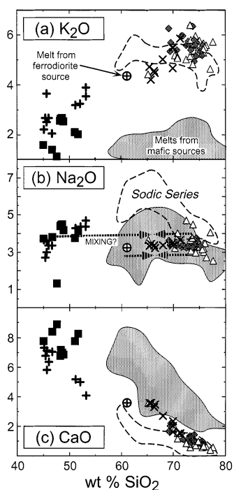
Fig. 10. (a) K_2O , (b) Na_2O and (c) CaO versus SiO_2 in Pikes Peak potassic granitoids and mafic rocks [symbols as in Figs. 3 and 4; data from this study and Barker et al. (1975)]. Dashed lines encircle compositions of Pikes Peak sodic granitoids. Shaded fields include compositions of melts generated from mafic source rocks; data from Holloway and Burnham (1972), Helz (1976), Spulber and Rutherford (1983), Rushmer (1991) and Beard and Lofgren (1991). Also shown is a melt composition (cross in circle) generated from a ferrodiorite source (Scoates et al., 1996).
