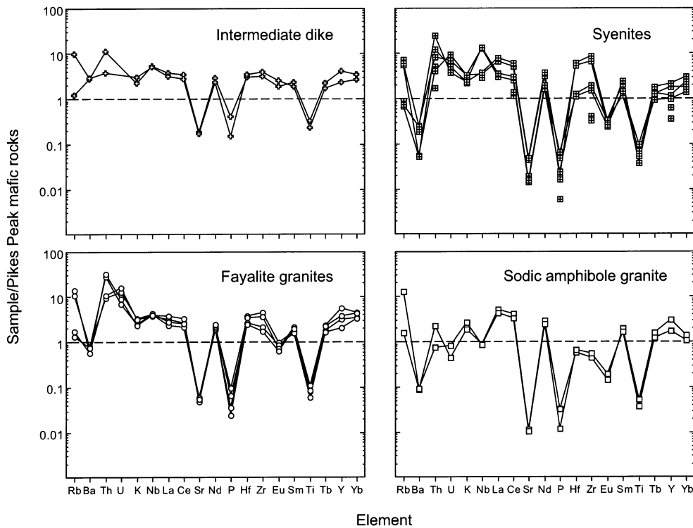
Fig. 12. Representative compositions of Pikes Peak sodic rocks normalized to representative Pikes Peak mafic rocks (gabbro sample CCN-19B-CD and diabase dike sample MBC-8-SG). Note the depletions in Ba, Sr, P, Eu and Ti, but enrichments in incompatible elements.
