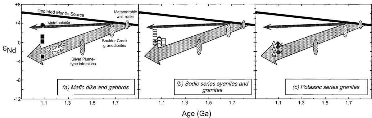
Fig. 9. \epsilon_{\text{Nd}} versus age relationships for (a) mafic dike and gabbros, (b) sodic series syenites and granites and (c) potassic series granites of the Pikes Peak batholith. The large arrow and black line show \epsilon_{\text{Nd}} evolution for typical 1.8 Ga Colorado crust and depleted mantle, respectively (from DePaolo, 1981a). The small arrow gives the \epsilon_{\text{Nd}} evolution for typical 1.8 Ga metatholeiitic basalt, and fields are shown for metamorphic wall rocks, Boulder Creek granodiorites and Silver Plume-type intrusions (from DePaolo, 1981a). In (b) and (c), data points are separated for clarity and no age differences are implied. Symbols as in Figs. 3 and 4.
