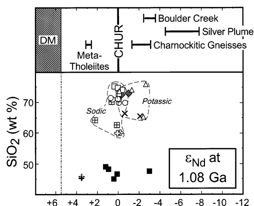
Fig. 8. \epsilon_{Nd} at 1.08 Ga versus SiO_2 (wt %) for samples of the Pikes Peak batholith (Table 11) and associated wall rocks (DePaolo, 1981a). An additional \epsilon_{Nd}(T) value of \sim 0 for the Silver Plume intrusions was omitted for clarity. Symbols as in Figs. 3 and 4.
