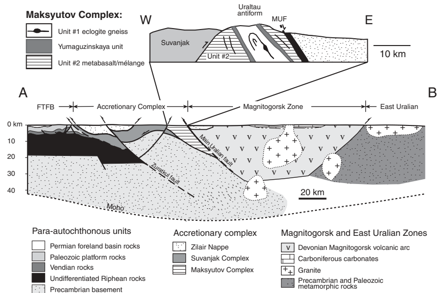
FIGURE 2. Schematic cross-section A-B across the South Ural Mountains, adapted from Brown et al. (1998) and Leech and Stockli (2000). See also Lennykh et al. (1995), Berzin et al. (1996), and Hetzel et al. (1998). An expanded cross-section through the Karayanova (Sakmara River) area details relationships among the units. MUF = Main Uralian fault; FTFB = foreland fold-and-thrust belt.
