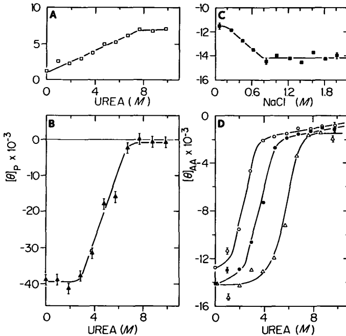
Figure 5. Circular dichroism of \nu_1 and inner histones at different urea concentrations. (A) [\theta]_{P,280} for \nu_1 . (B) [\theta]_{P,222} for \nu_1 . (C) [\theta]_{AA,223} for inner histones as a function of NaCl molarity. (D) [\theta]_{AA,223} for inner histones as a function of urea molarity, in 0.4 (O), 1 (●), and 2 M ( \Delta ) NaCl containing 0.1 mM DTT and 10mM Tris (pH 7.0).
