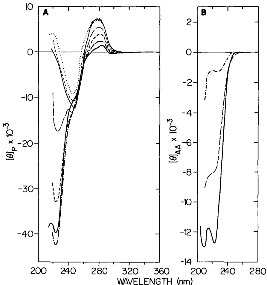
Figure 4. Circular dichroism of \nu_1 and of inner histones at different urea concentrations. (A) \nu_1 in 0 (—), 2 (—○—), 4 (----), and 6 M urea (—□—), (thin lines), and in 8 (-·-·-) and 10 M urea (thick lines), containing 0.2 mM EDTA (pH 7.0). Chicken DNA (.....) in 0.1 M NaCl [\theta]_p , molecular ellipticity per mole nucleotides. (B) Inner histones in 0 (—), 6 (---), and 9 M (—○—) urea containing 2 M NaCl, 0.1 mM DTT, and 10 mM Tris (pH 7.0) [\theta]_{AA} , molecular ellipticity per mole histone amino acid residues.
