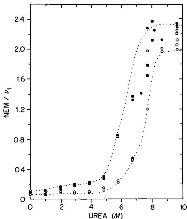
Figure 6. Reaction of ^3\text{H} -labeled NEM with \nu_1 as a function of urea molarity. Samples: \nu_1 (■), different preparations of total \nu_1 (○, ○, □). NEM/ \nu_1 measured in moles of NEM/mole of \nu_1 .
